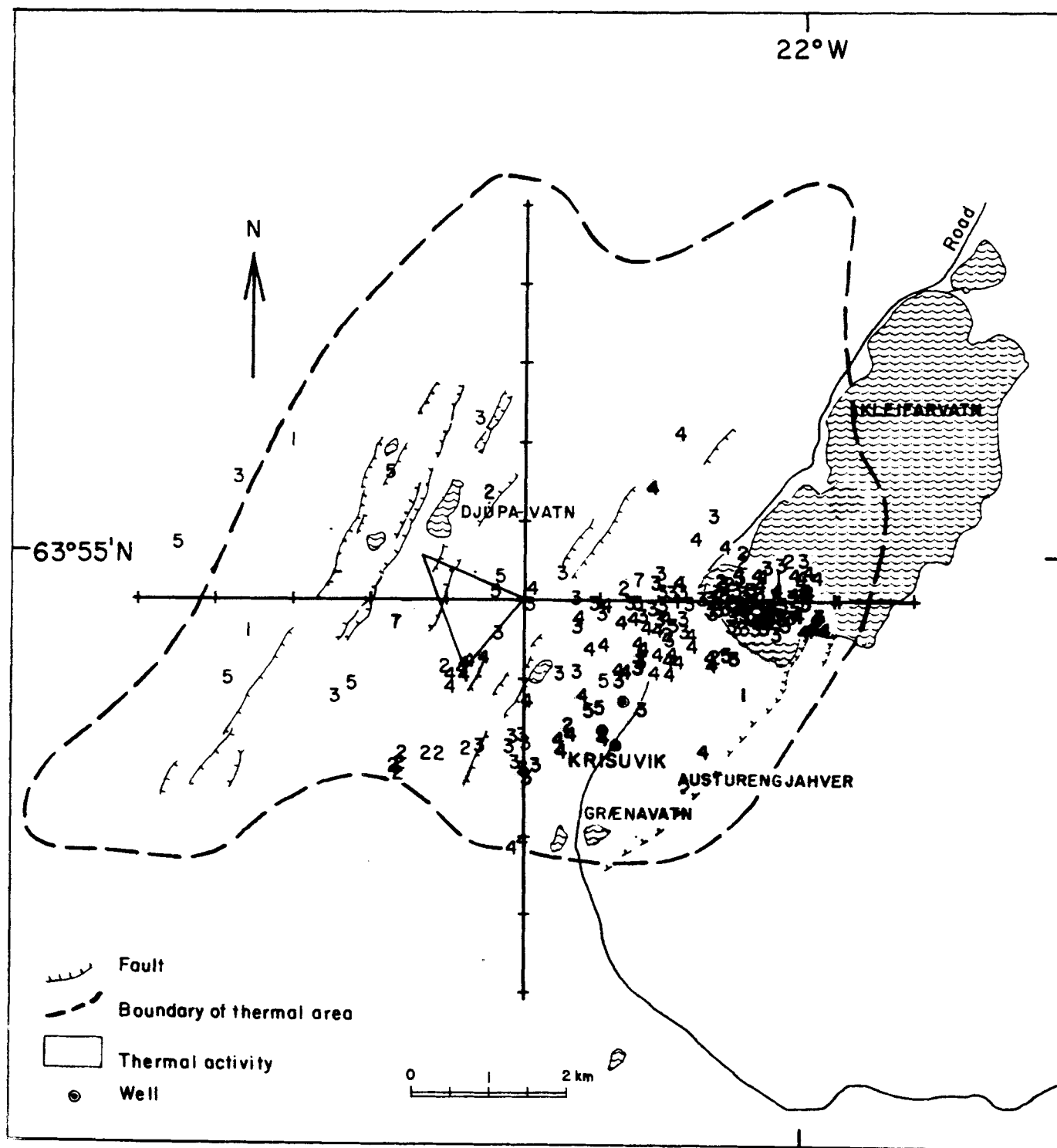
FIG. 1. — Locations of earthquakes in the Krisuvik geothermal area, 25 km south-southwest of Reykjavik, Iceland. The numbers are hypocentral depths rounded to the nearest kilometer. The earthquakes were located using the tripartite area shown south of Djupavatn. The dashed line shows the horizontal extent of thermal alteration observed at the surface.
