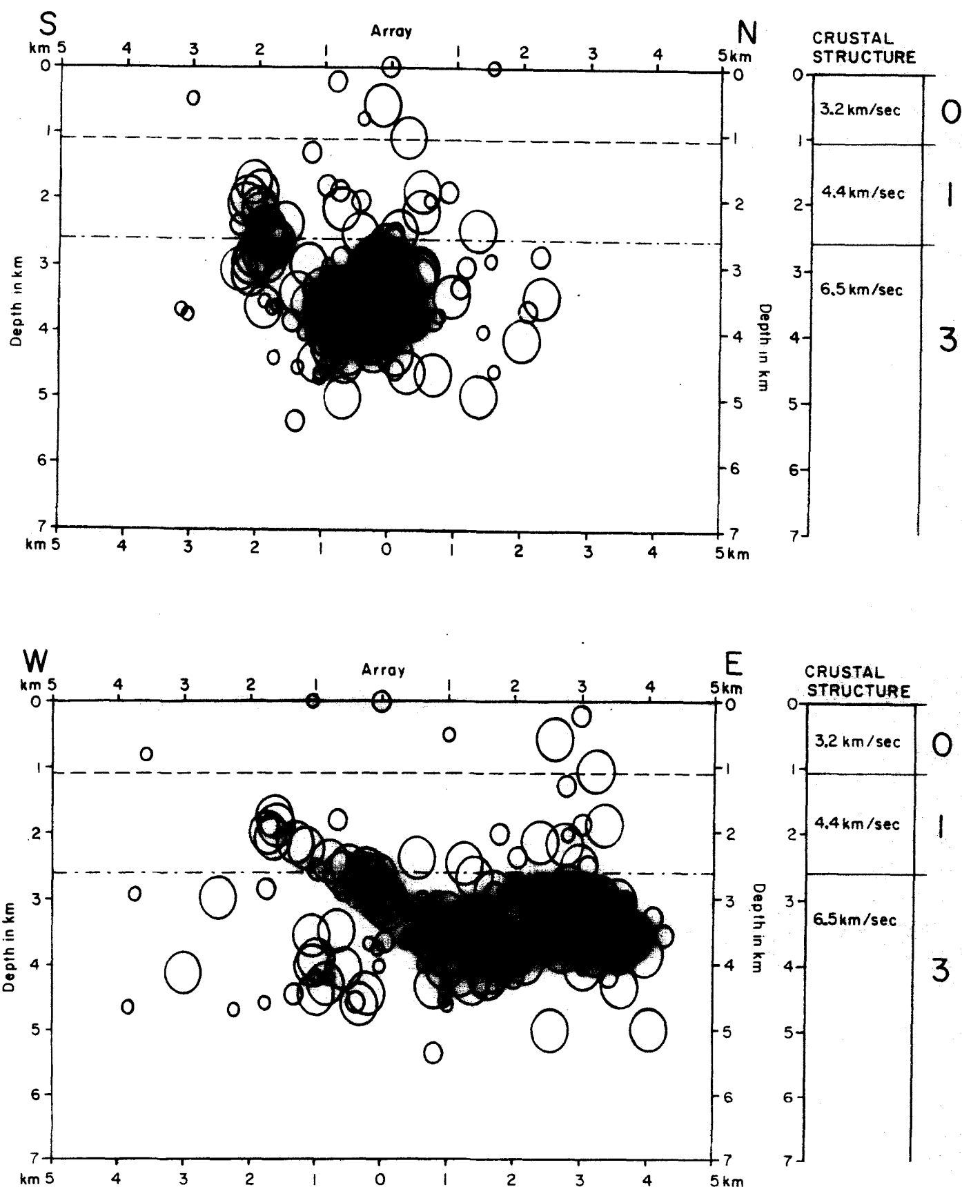
FIG. 2. — Earthquake hypocenters in Krisuvik projected onto north-south and east-west vertical cross-sections drawn along the axes in Figure 1. The crustal structure is from PÁLMASSON (1971).
